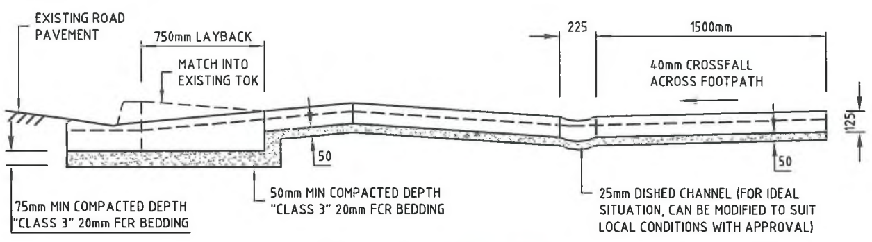
SECTION A-A (REVERSE FALL) (ONLY TO BE USED WITH COUNCIL APPROVAL)
