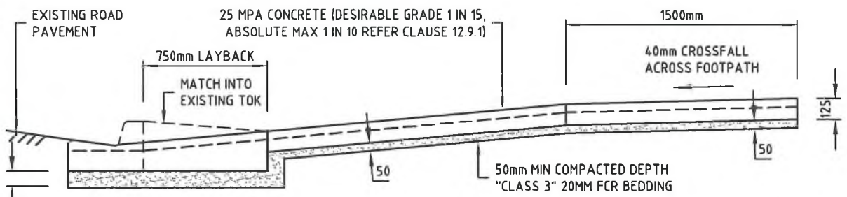
SECTION A-A (STANDARD)
